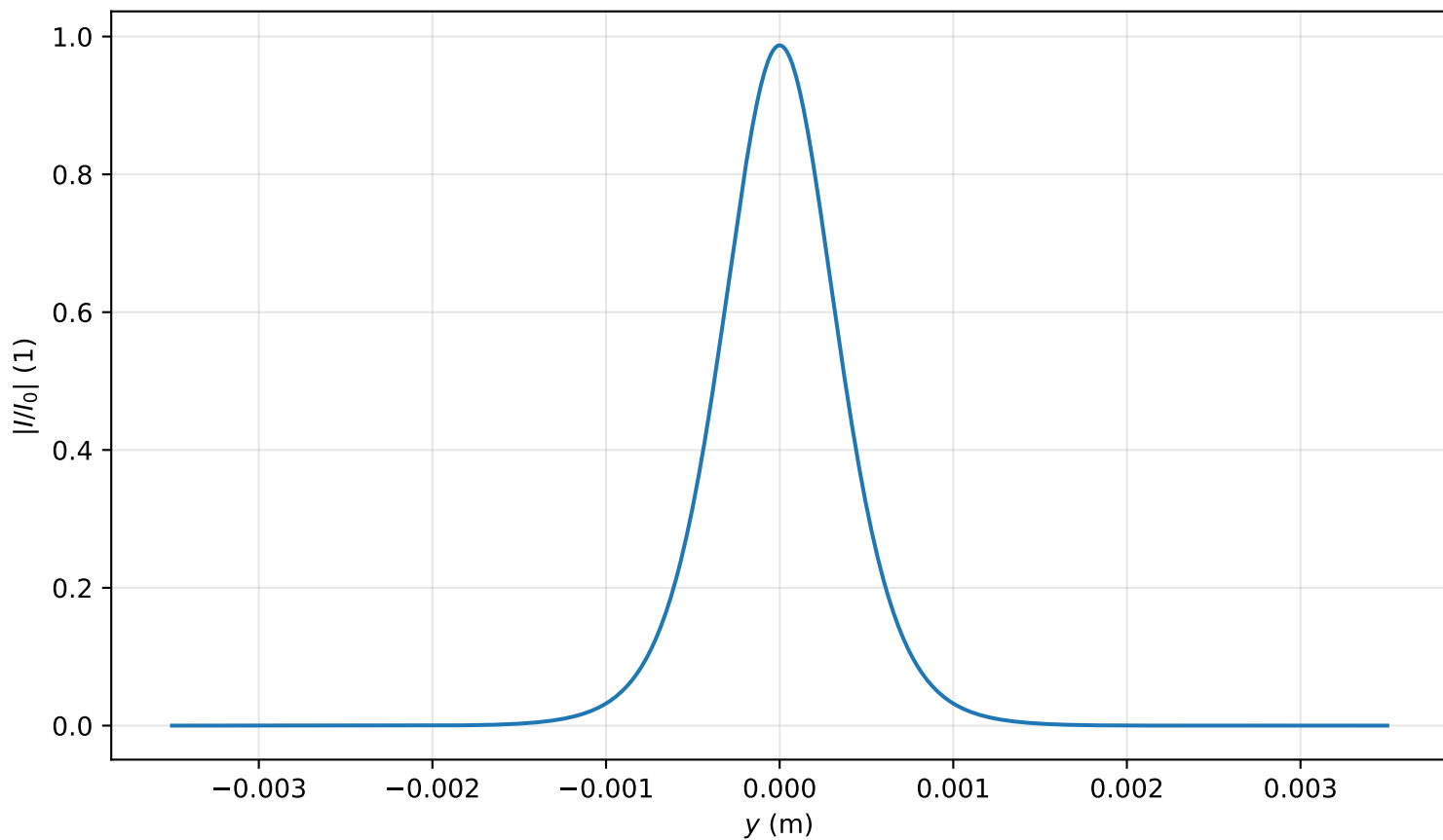
Intensity profile I(x=0, y, z=1.831)/I_0 , \text{Pin}=0.6\text{Pcr} , artificial time
